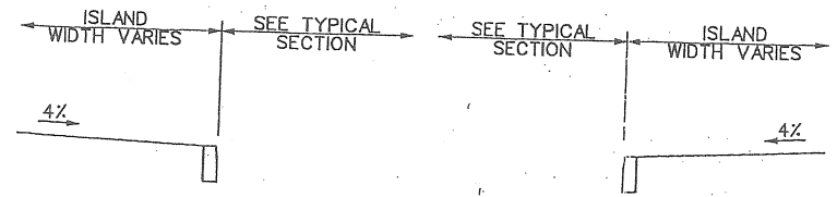
SR 0063 (WELSH ROAD) TYPICAL ISLAND TREATMENT STA 32+27.96 TO STA 33+39.52 LEFT STA 35+33.82 TO STA 36+41.18 RIGHT NOT TO SCALE
